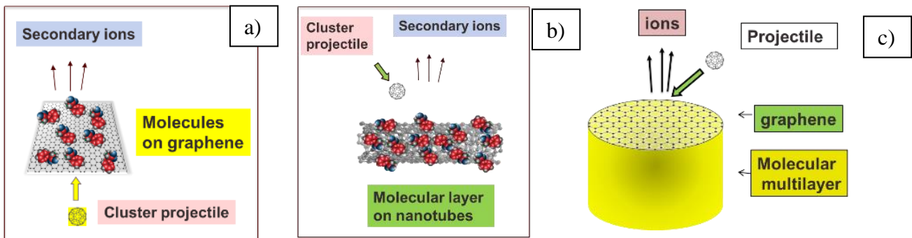
Figure 1. Sketch of bombardment/emission directions. a) sub-single molecular layer of Phe molecules deposited on 2L graphene; b) sub-single layer of Phe molecules on multi-wall carbon nanotubes; c) a polymer layer of PMMA (~1 mm) covered by a single-layer 13 C graphene.
