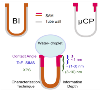
(a) Schematic illustrating functionalization depths for nanotubes modified via BI and \mu CP
