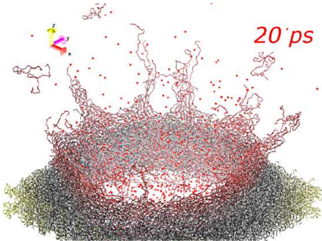
Figure. Perspective view of the crater forming in a polymeric surface following a 10 keV Ar 1000 impact at normal incidence (Time: 20 ps – Red dots are Ar atoms).
