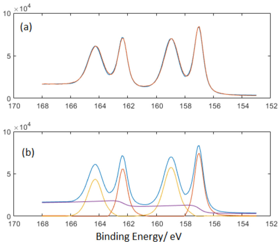
Redox XPS results for Bi 4f peaks. XPS narrowscan spectra (a) measured data in red and automatically-fitted data in blue, and (b) components of the automatic fit in red and orange, on fitted background in purple.
