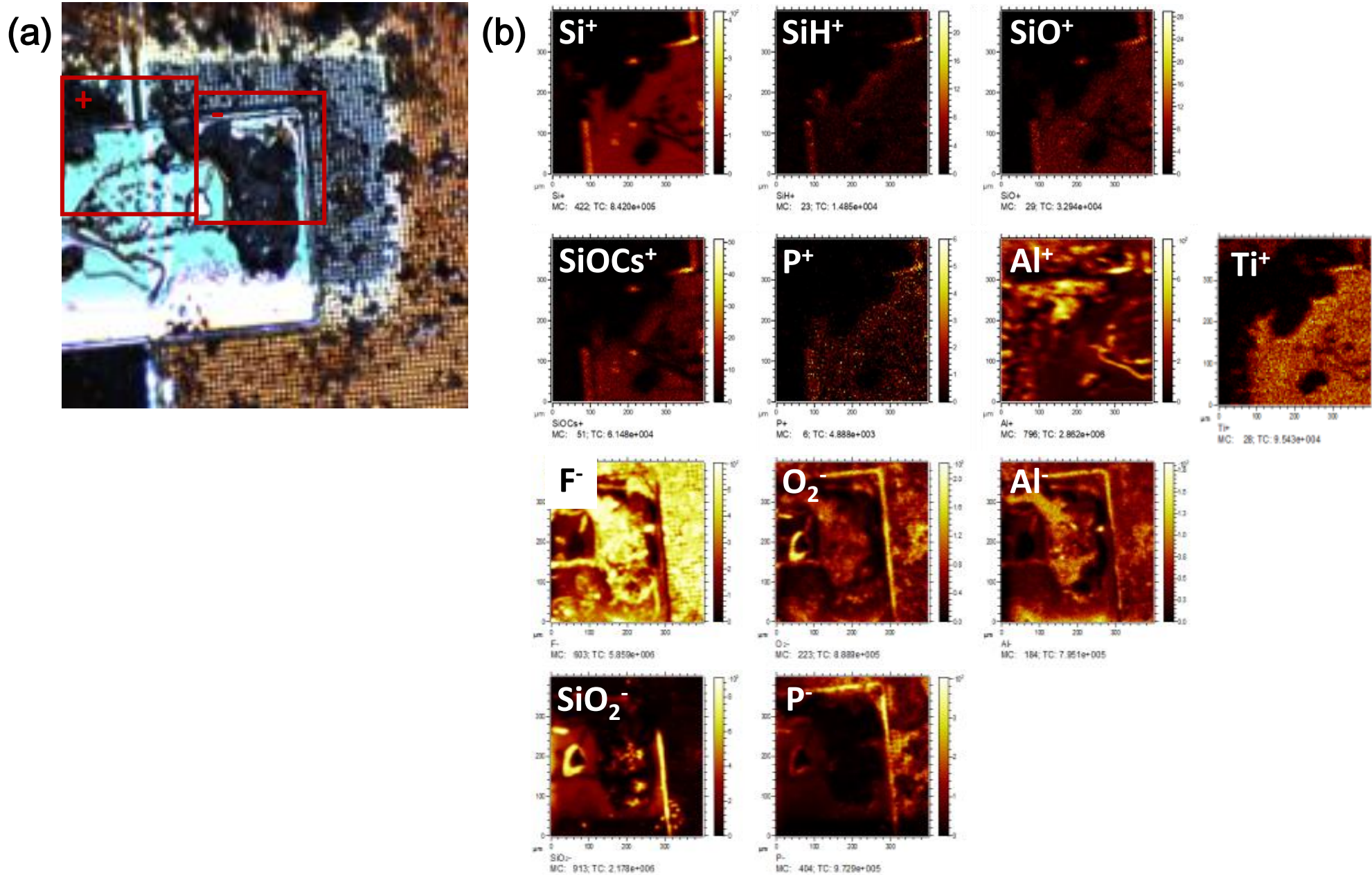
Figure 1 (a) Failed region in device, and (b) positive and negative ion map of each element. The red squares indicate the analysis region.
