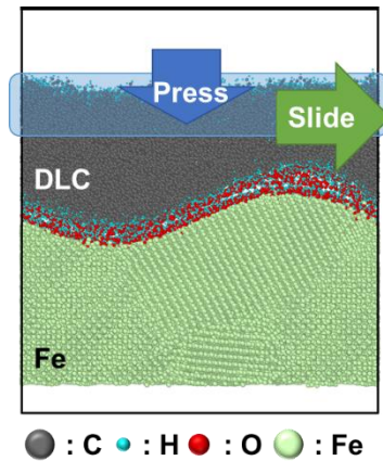
Fig.1 Sliding simulation model of DLC/Fe.
