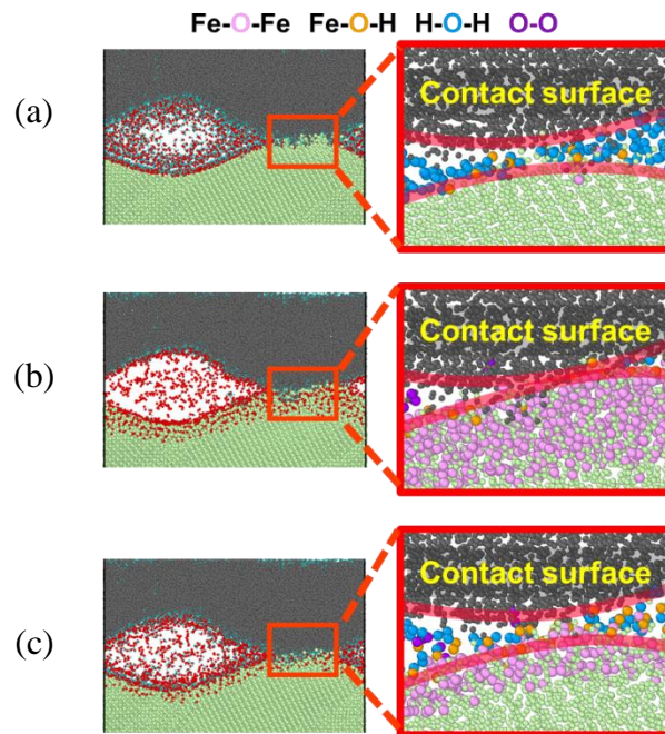
Fig.2 Snapshots of the sliding simulations for (a) H 2 O model (b) O 2 models and (c) H 2 O+ O 2 model at 50 ps. O atoms are shown by different colors. Magenta, orange, blue, and purple balls indicate O atoms in Fe-O-Fe group, Fe-OH group, H 2 O molecule and O 2 molecule, respectively.
