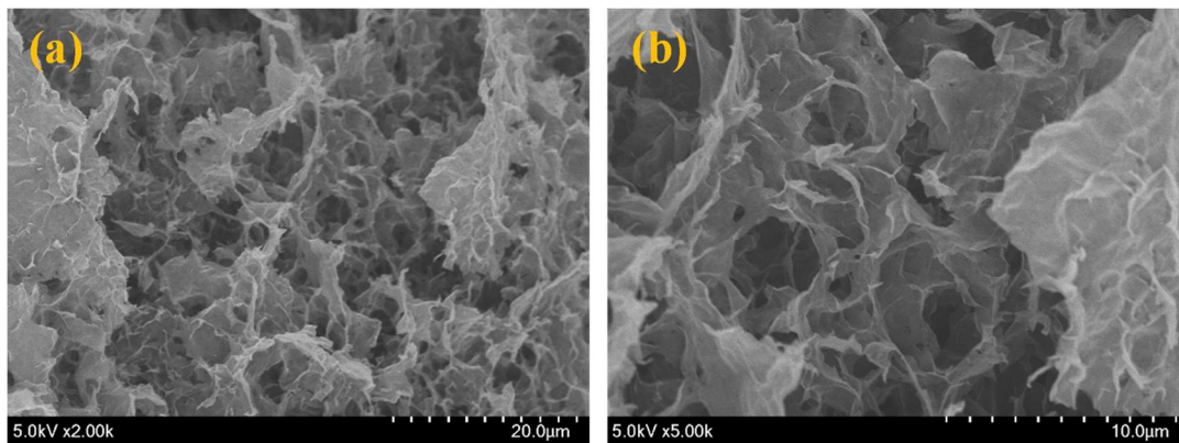
Figure 2. SEM images of 3D foams with different surfactants (a) and surface morphology of the internal cellular structures of 3D foams (b).
