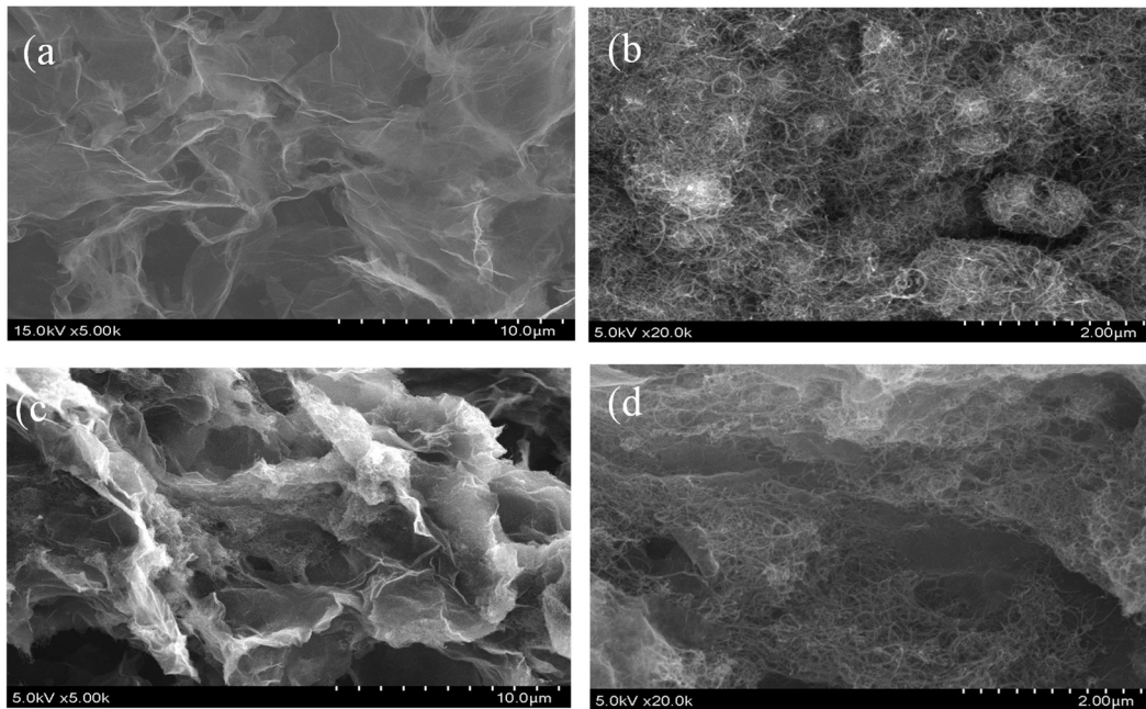
Figure 1. SEM images with different magnification of MWCNT/rGO hybrid nanofillers. (a) rGO, (b) MWCNT, (c) and (d)
