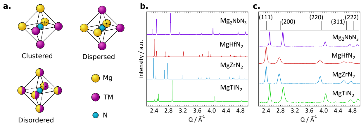
Figure 1: Structural properties of Mg_{G-3}TMN_{G-2} (TM=Ti, Zr, Hf, Nb) materials.
