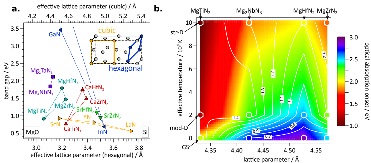
Figure 3: Tunable properties of Mg_{G-3}TMN_{G-2} semiconductors. (
