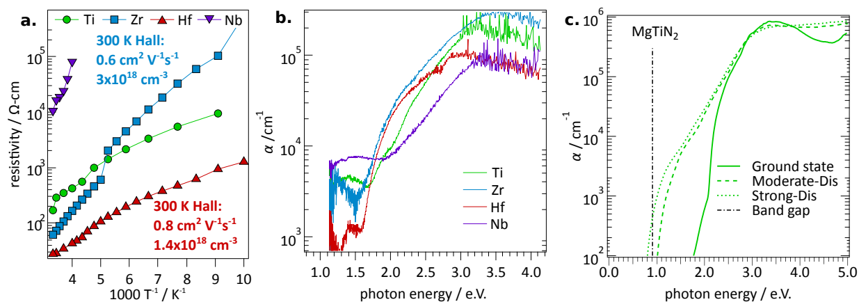
Figure 2: Optoelectronic properties of Mg_{G-3+x}TM_{1-x}N_{G-2} materials.
