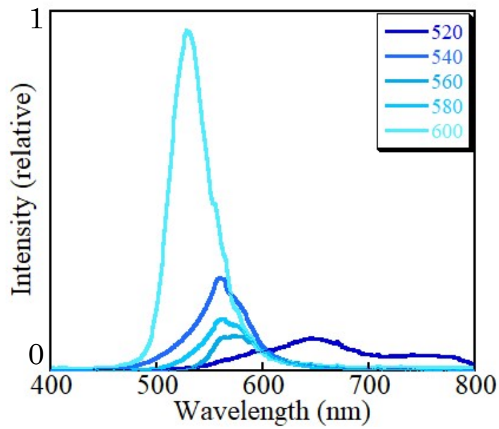
Fig.2 PL measurement by growth temperature
