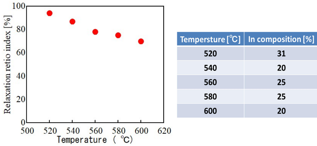
Fig1. Relationship between temperature and relaxation ratio index and In composition.
