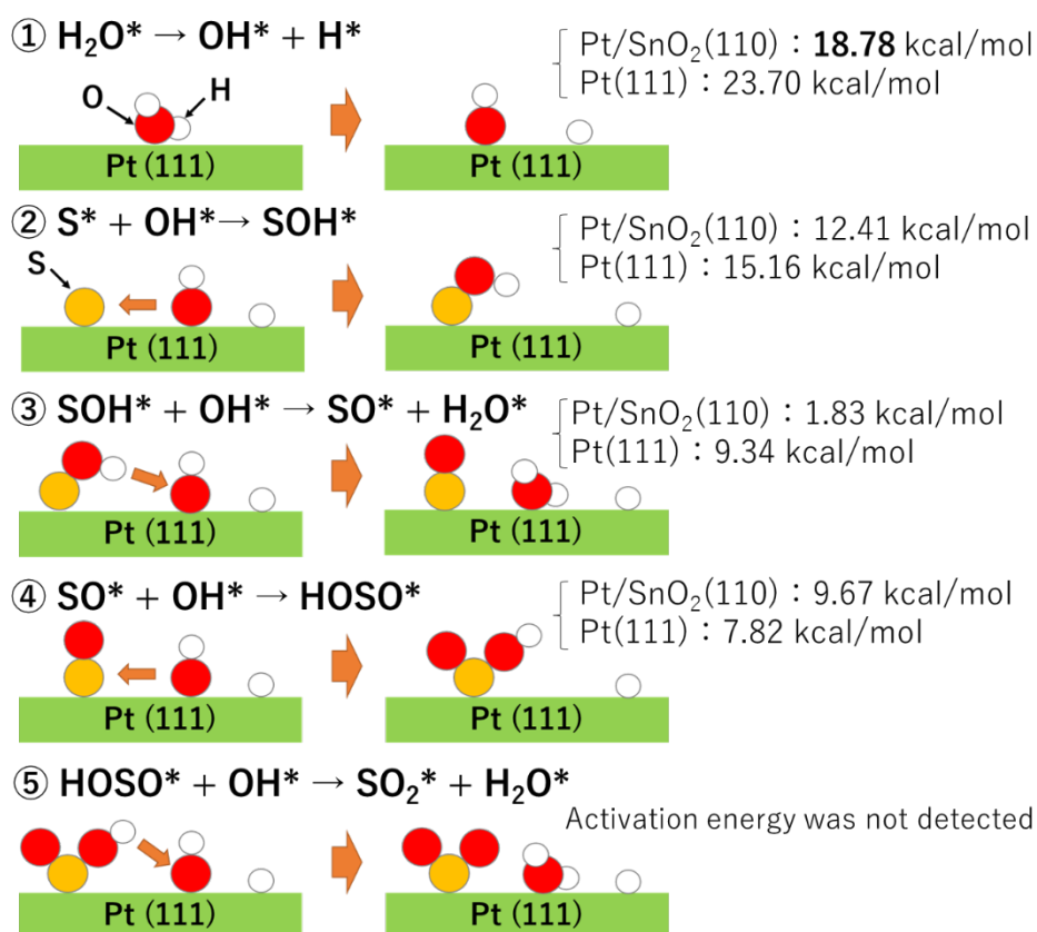
Fig. 2 Oxidation reaction process of adsorbed sulfur atom by H 2 O molecule and activation energy for each elementary process
