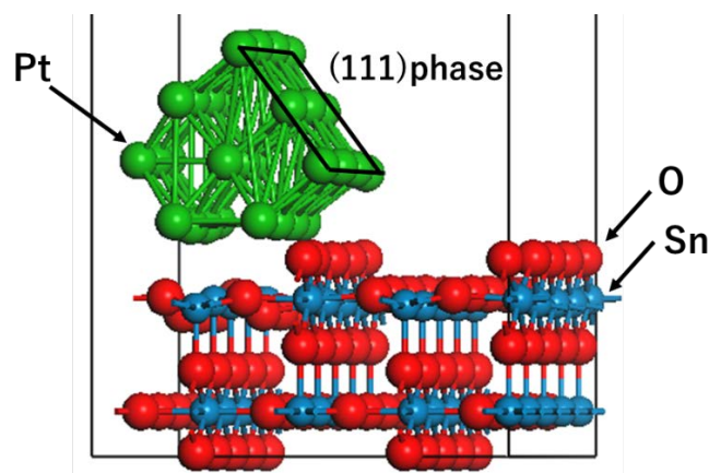
Fig. 1 Pt/SnO 2 (110) model
