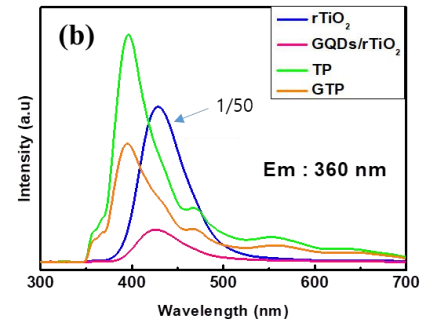
[PL spectra of (a) GQDs/TiO 2 , and (b) GQD/TiO 2 /PAN]
