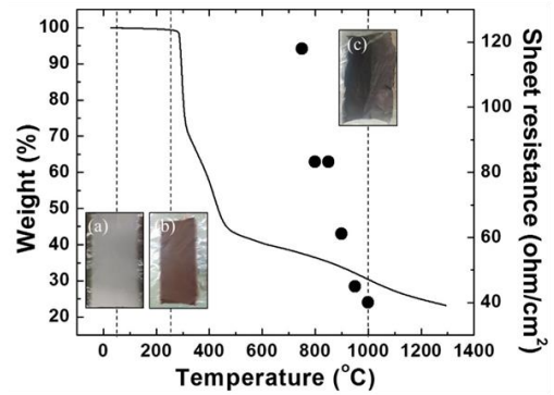
[TGA result and electrical conductivity of PAN-CFs]
