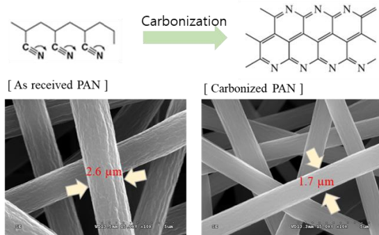
[Schematic diagram of PAN and SEM images of electrospun PAN-CFs before and after heat treatment]
