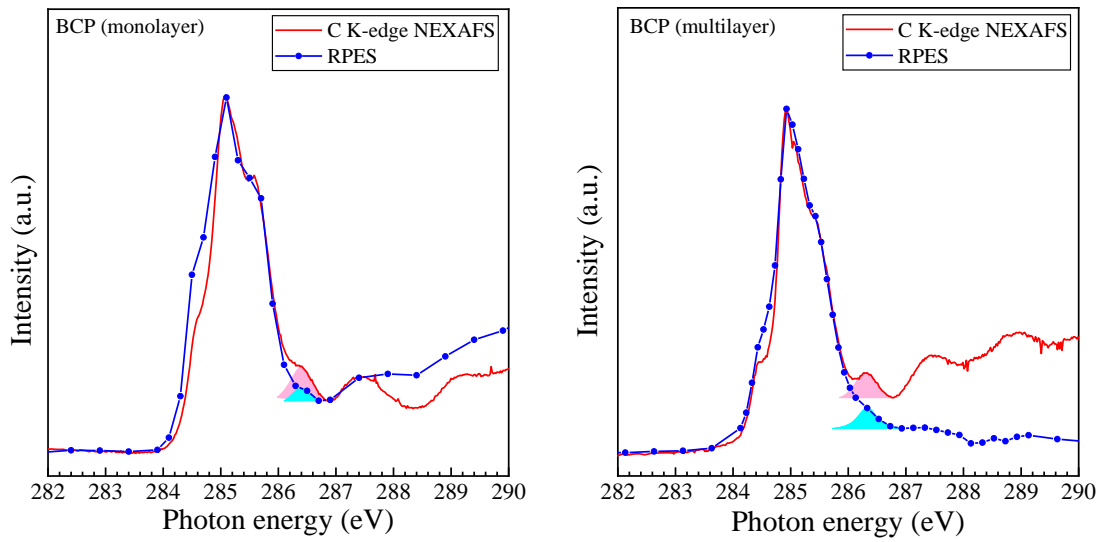
Fig. C K-edge NEXAFS and RPES spectra of BCP on Ag.
