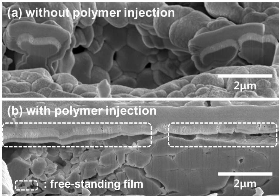
Figure 2 Cross sectional images of thin film on porous NiO-YSZ substrate (a)without polymer injection (b)with polymer injection observed by FIB-SEM
