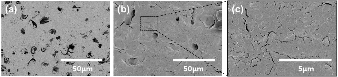
Figure 1 Surface morphology of thin film on porous NiO-YSZ substrate (a)without polymer injection (b,c)with polymer injection observed by FE-SEM
