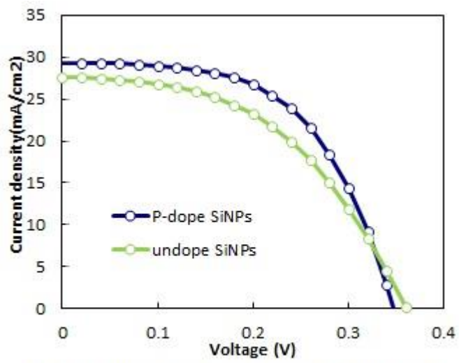
Fig. 1 J - V characteristics of undoped and P-doped SiNPs/PEDOT:PSS solar cells
