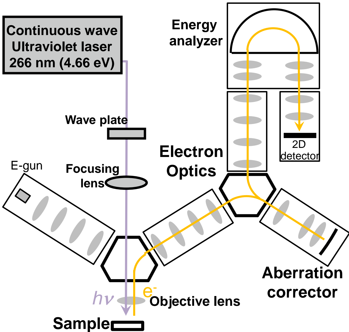
Figure 1: Schematic of the Laser-PEEM system.
