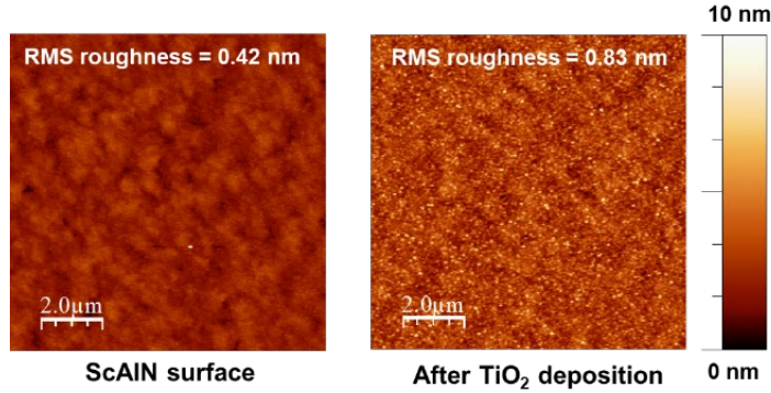
Fig. 1 AFM images of ScAlN surface of ScAlN HEMT structure before and after TiO 2 deposition.
