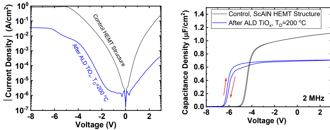
Fig. 2 Vertical I-V and C-V of ScAlN HEMT structure with Schottky contact (black line) compared to structure with ALD TiO 2 (blue line).
