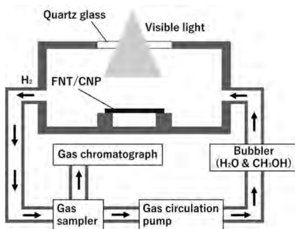
Fig. S1. Schematic drawing of experimental setup for monitoring gas phase photocatalytic hydrogen production over the CNP/FNT sample.
