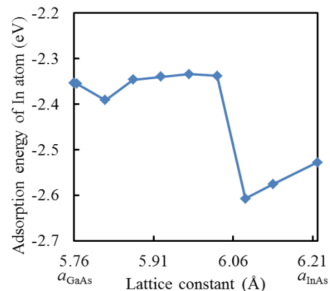
Fig. 1. Calculated adsorption energy of In atom on the (4×3) reconstructed surface including In-As dimers as a function of hypothetical lattice constant of the InAs WL. a_{\text{GaAs}}=5.76 and a_{\text{InAs}}=6.21 Å are calculated lattice constant of bulk-GaAs and InAs, respectively.
