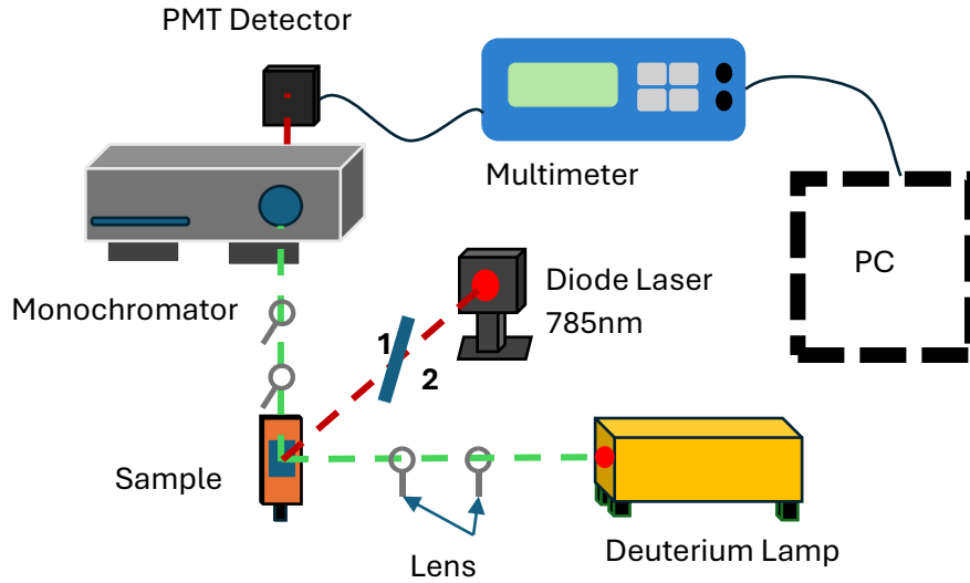
Figure 1. Experimental setup of the thermal modulation spectroscopy technique employed to obtain the bandgap energy.
