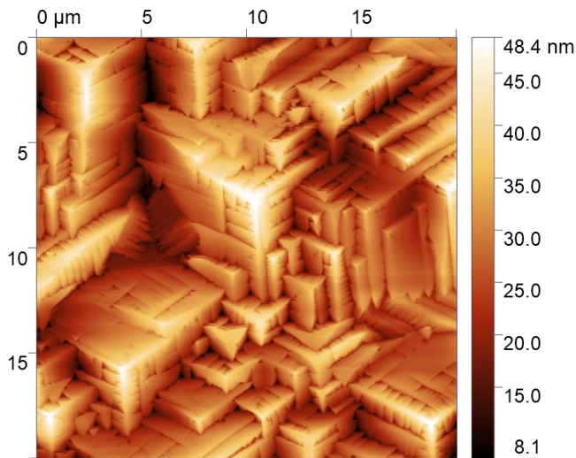
Characteristically rough GaSb (111)A
