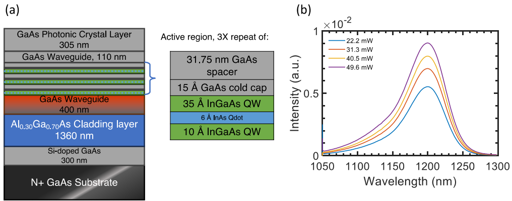
Fig. 1. (a) Initial growth structure, (b) Photoluminescence measurement from initial growth structure.
