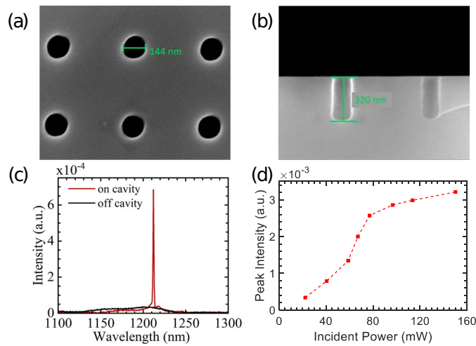
Fig. 3. (a) Top down (b) Cross sectional SEM image of PCSEL devices (c) Photoluminescence emission measurement from PC off cavity (black) and on cavity (red) and (d) L-L curve.
