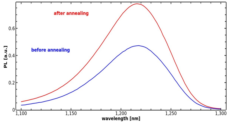
Fig. 2. Photoluminescence of initial growth structure before and after annealing, which simulates the thermal effect of the regrowth.
