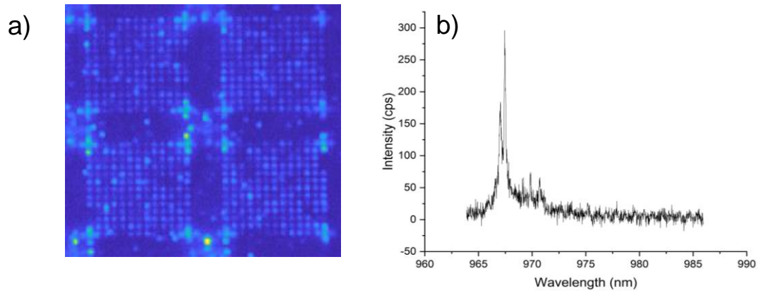
Figure 1 – a) PL imaging of site-controlled QD array, b) micro-PL spectra of site-controlled QD emission
