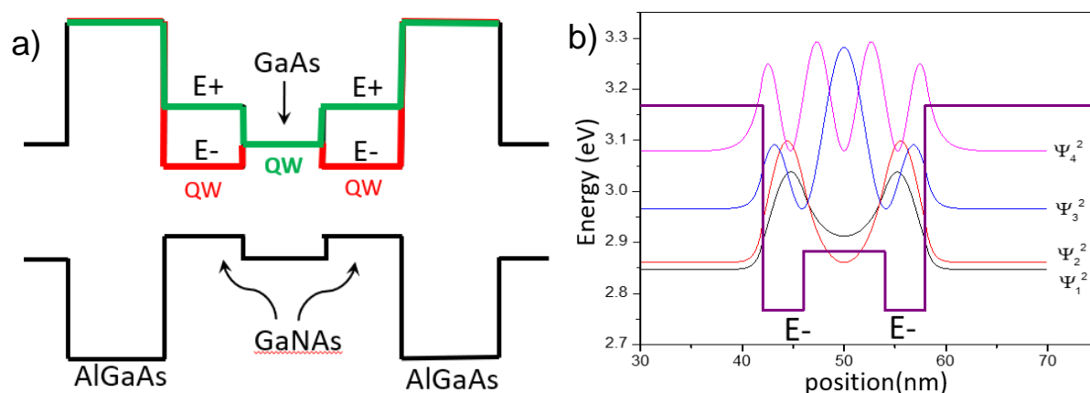
Figure 1. a) Schematic band structure of the GaNAs multi-quantum well heterostructures investigated in this work. b) Probability density of the eigenstates confined within the AlGaAs barriers.
