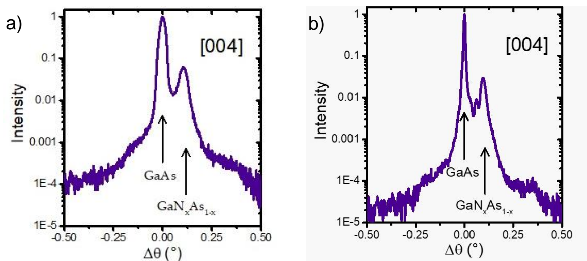
Figure 2. HRXRD patterns of the multi-quantum well heterostructures with a) x=0 and b) x=30\% AlGaAs.
