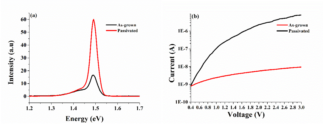
Figure 1: (a) 4K PL (b) room temperature (RT) I-V of as-grown and hydrazine treated GaAs NW.
