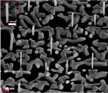
Figure 1 SEM image of \text{GaAs}_{1-x}\text{Sb}_x ( x = 0.1 ) NWs grown on graphene.
