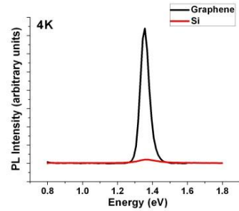
Figure 2 4K \mu - photoluminescence spectra of single nanowire (SNW) grown on graphene and Si substrates.
