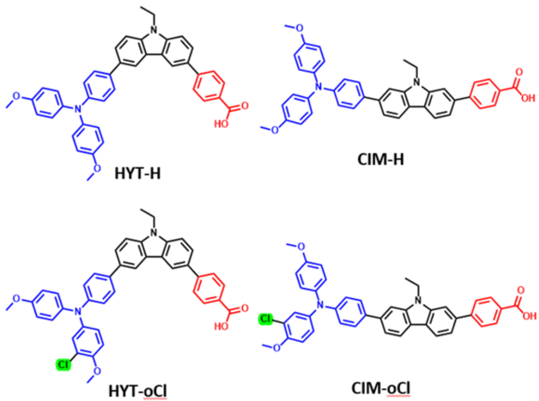
Fig. 1. Molecular structures of Self-Assembling Monolayers (SAMs)
