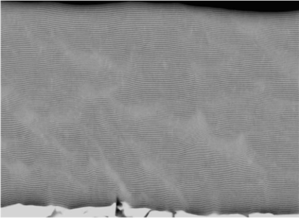
SEM micrograph of multilayered HEN-MN coating deposited using 100V of deposition bias volage.
