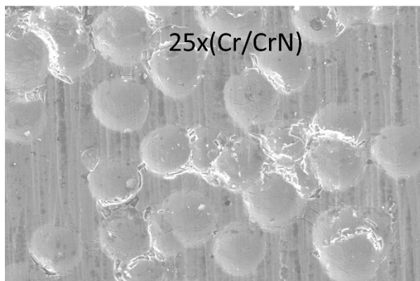
Randomised impact testing for simulating solid particle erosion
