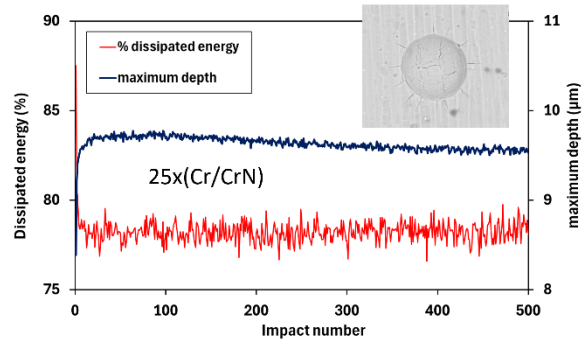
Cyclic micro-impact testing for simulating machining
