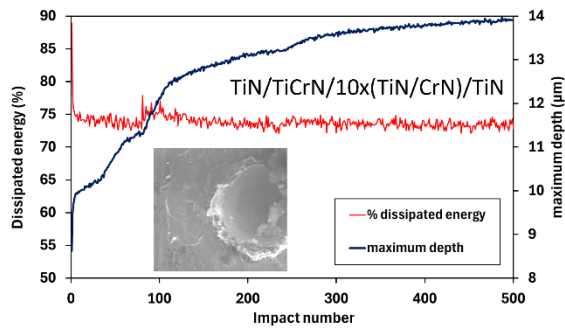
Cyclic micro-impact testing for simulating machining
