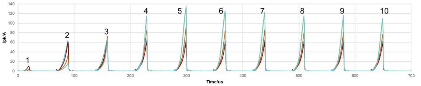
Fig 2. Current waveforms with changing O 2 flow @Multi-pulse HiPIMS
