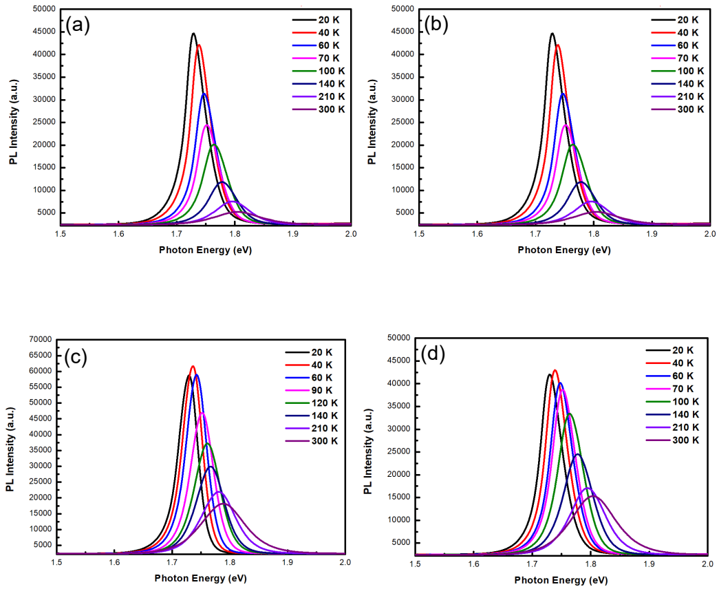
Figure 1. Temperature dependent photoluminescence spectra for CsPbI 3 QD thin films with (a) 0%, (b) 3%, (c) 5%, and (d) 7.5% Zn doping concentration.
