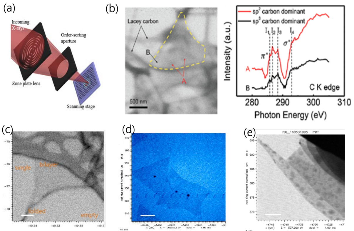
Figure 1 (a) Soft x-ray STXM. (b) Graphene oxide. sp^2 , sp^3 distribution. (c) Graphene. (d) MoS_2 . (e) Black phosphorus. Oxidized surface.
