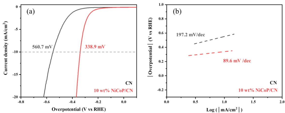
Figure 2. Electrochemical performance of g-C 3 N 4 and 10 wt% NiCoP/ g-C 3 N 4 .
