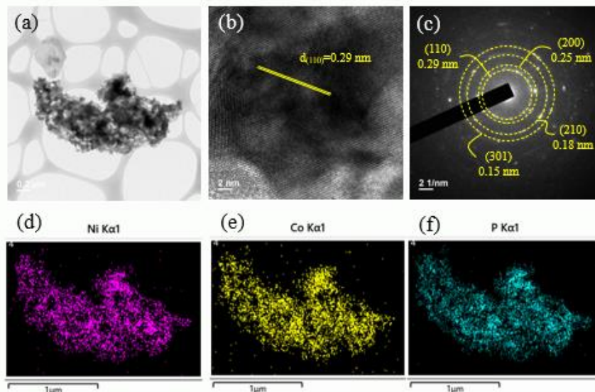
Figure 1. (a) TEM image, (b) HRTEM image, (c) SAED image, and (d)(e)(f) EDS mapping images of 10 wt% NiCoP/g-C 3 N 4 .
