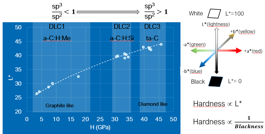
Figure 1. Transparency (defined by L^* values) of carbon-based coatings as a function of hardness.
