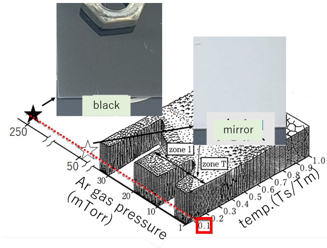
Figure 1 Al films obtained in the study which are overlaid on the structure zone model
