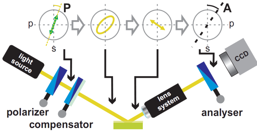
Figure 1. Schematic of Imaging Spectroscopic Ellipsometer (ISE) in PCSA configuration.
