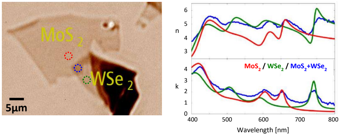
Figure 2. Characterization of local complex refractive indices for MoS 2 and WSe 2 heterostructures
