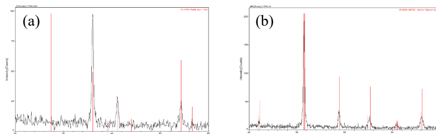
Fig. 1 XRD diagram of (a) \text{TiO}_2 (b) \text{BaTiO}_3
