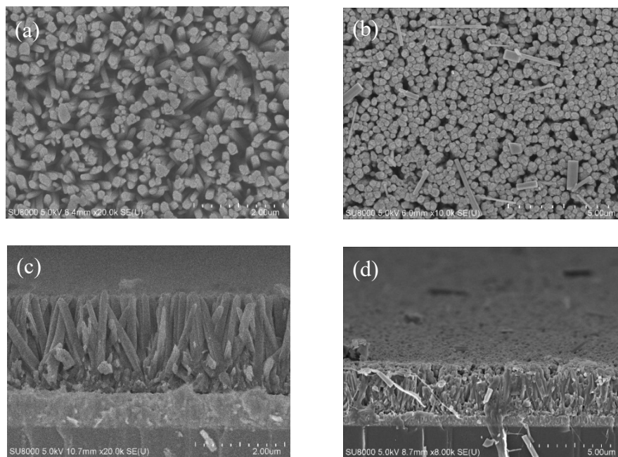
Fig. 2 Top view of SEM graphs of (a) \text{TiO}_2 (b) \text{BaTiO}_3 and cross-sectional view (c) \text{TiO}_2 (d) \text{BaTiO}_3
