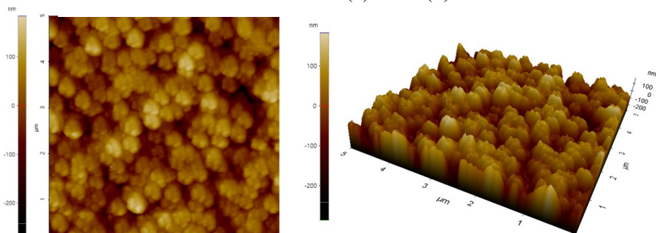
Fig. 3 Topography of \text{BaTiO}_3 nanorod arrays from (a) 2D (b) 3D graph
