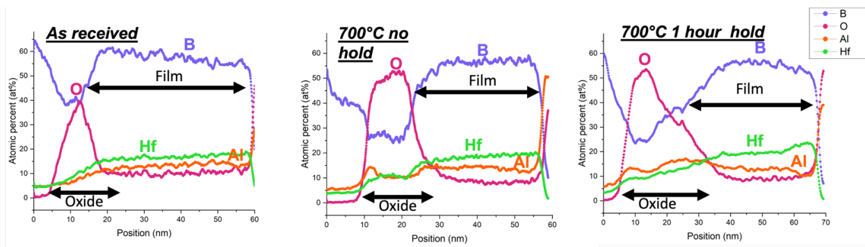
Fig 1: Composition profiles, depicting the change in composition of the coating across its depth, obtained from EDS maps. The hafnium, aluminum and boron content within the coating is uniform, and does not change after any heat treatment. For the oxide, the aluminum content in the oxide increases due to the hold at 700°C
