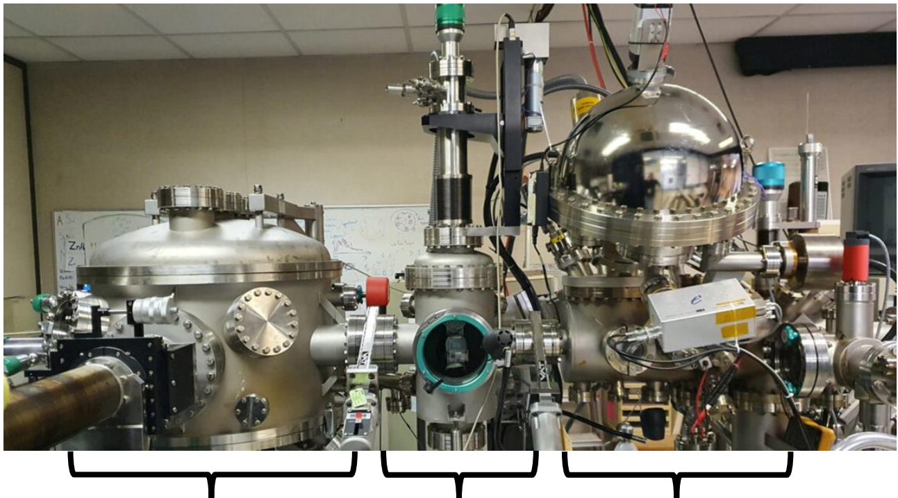
Deposition chamber & Real-time measurements
