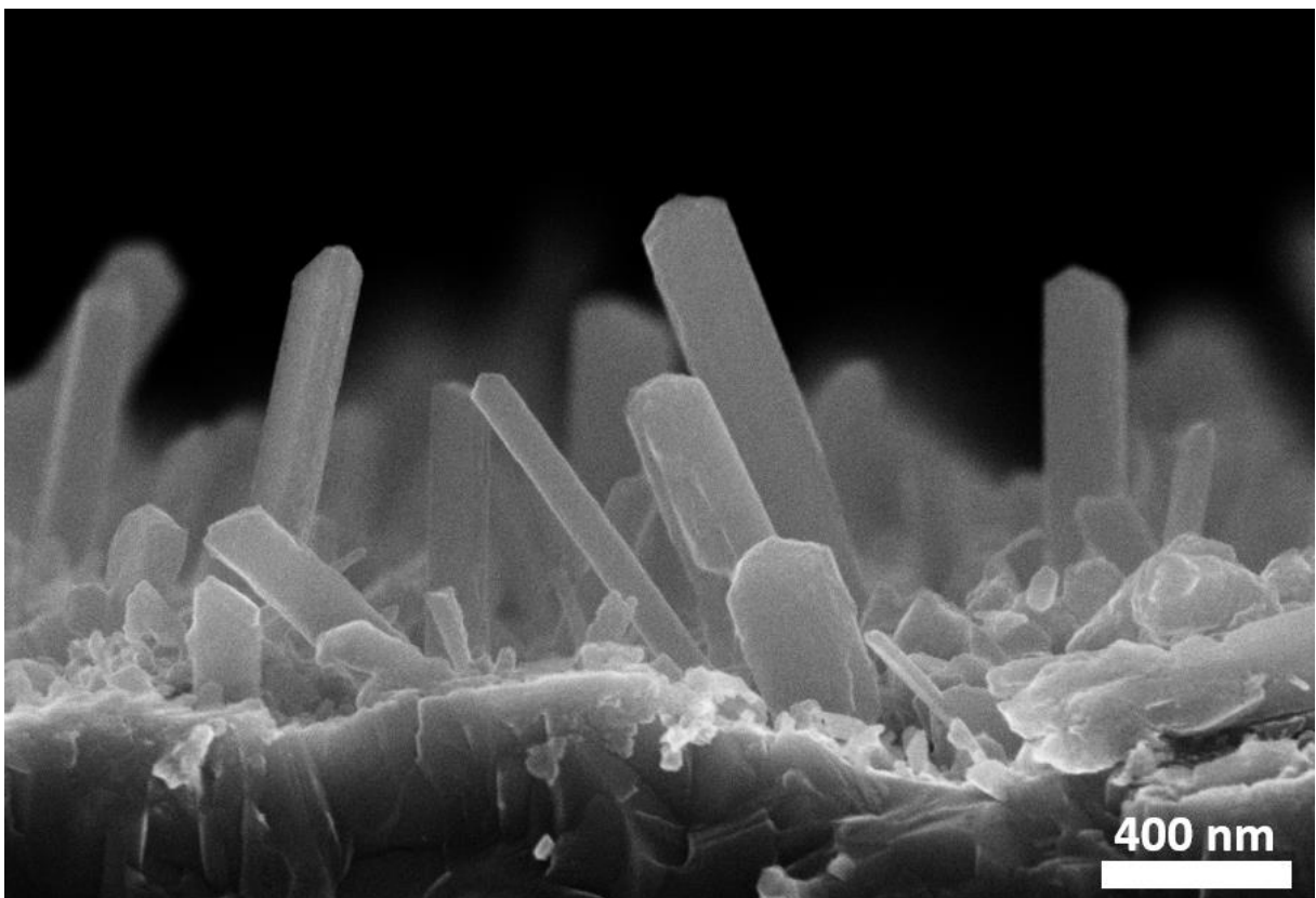
Figure 2 SEM cross-sectional image of the Mg nanowire coating.
