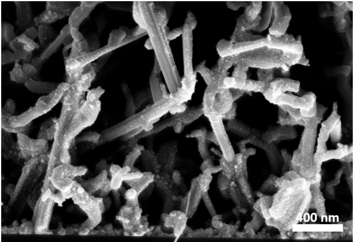
Figure 1 SEM cross-sectional image of the Zn nanowire coating.
