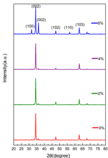
Fig. 1. XRD results of VZnO nanorods grown by 0-6 V% growth solution.
