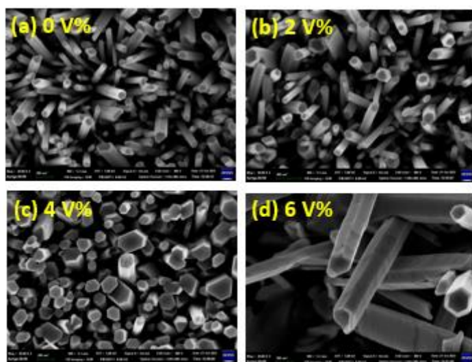
Fig. 2. SEM top-view images of VZnO nanorods grown by (a) 0 v% , (b) 2 v% , (c) 4 v% , (d) 6 v% growth solution.
