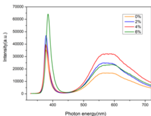
Fig. 3. Photoluminescence spectrum of VZnO nanorods grown by 0-6 V% growth solution.
