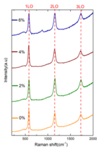
Fig. 5. Resonance Raman spectrum of of VZnO nanorods grown by 0-6 V% growth solution.
