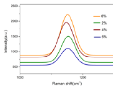
Fig. 6. The 2LO peak of the PL spectrum.
