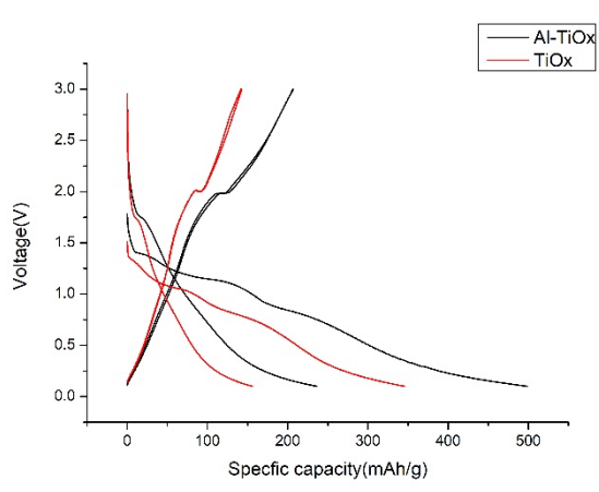
S3. First and second cycle of batteries
