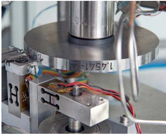
Sample configuration for cryogenic tribotests
