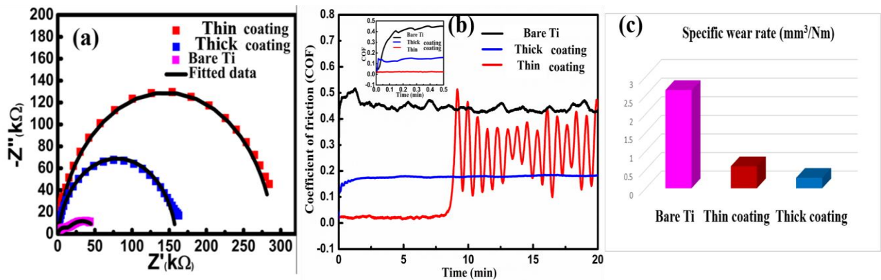
Fig. 2 (a), (b) and (c) shows Nyquist plot, plot of COF versus sliding time curves and specific wear rate of bare titanium substrate, thin and thick graphene-coated samples respectively.
