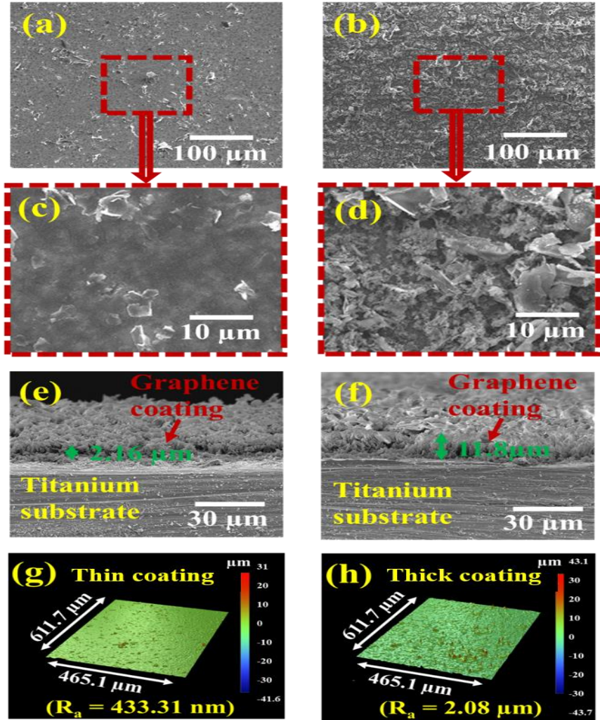
Fig. 1 Surface morphologies of (a) Thin coating; (b) Thick coating and their corresponding high magnification images (c) and (d); cross-sectional SEM images (e) and (f); surface topographies (g) and (h) respectively.
