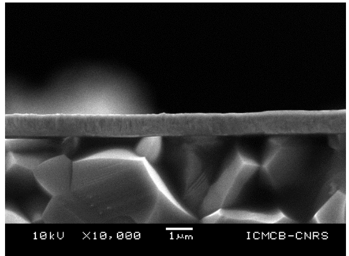
SEM photograph of TaN thin film by HiPIMS
