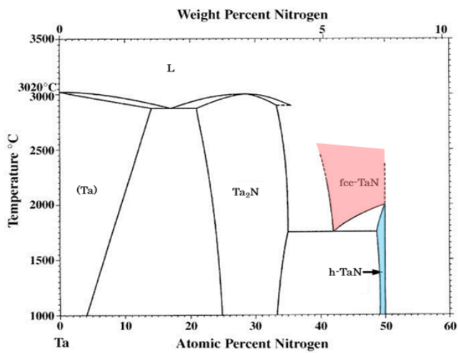
Ta-N phase diagram [1]
