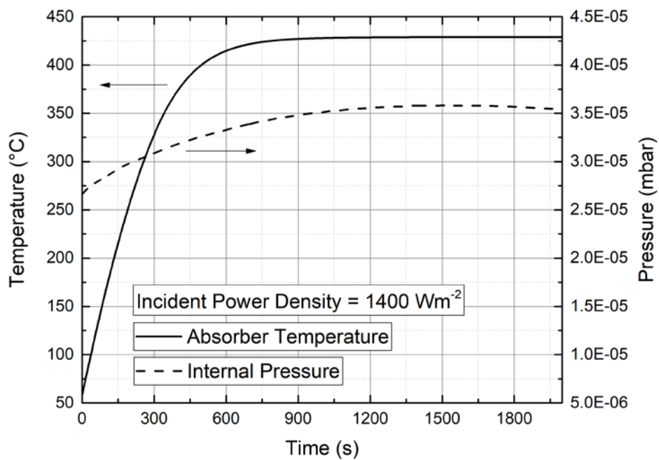
Figure 2 - The absorber temperature and the internal pressure during a calorimetric test are reported as function of time.
