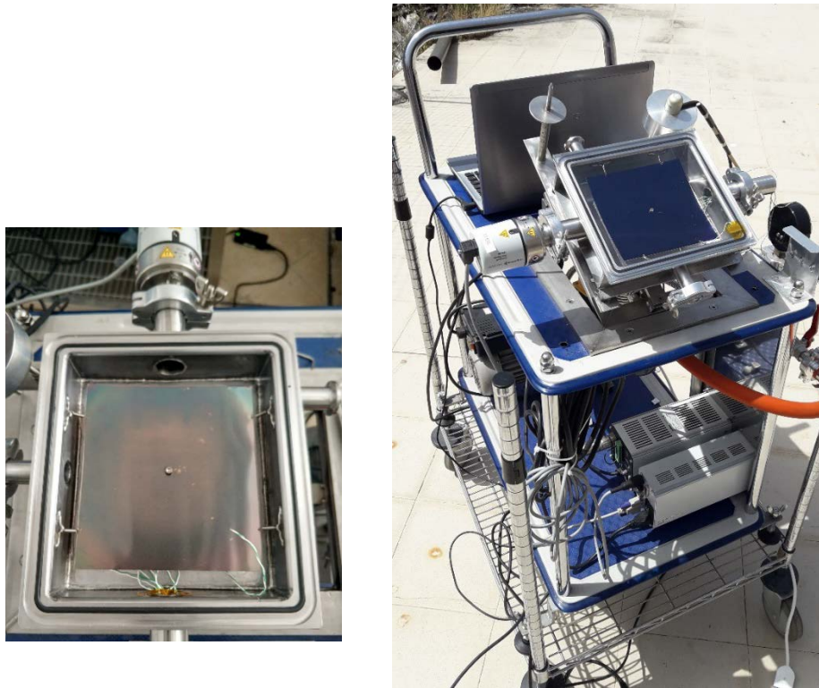
Figure 1 - Left: A Selective Solar Absorber is installed in the calorimetric device. Right: The calorimetric device during the outdoor testing procedure
