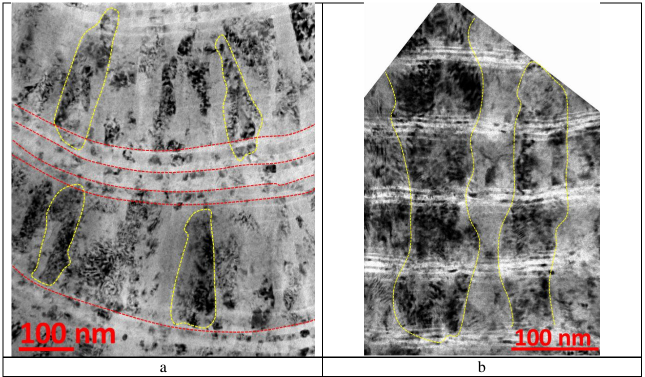
Influence of interlayer boundaries on the growth of crystals in coatings (a) K1 and (b) K3.
