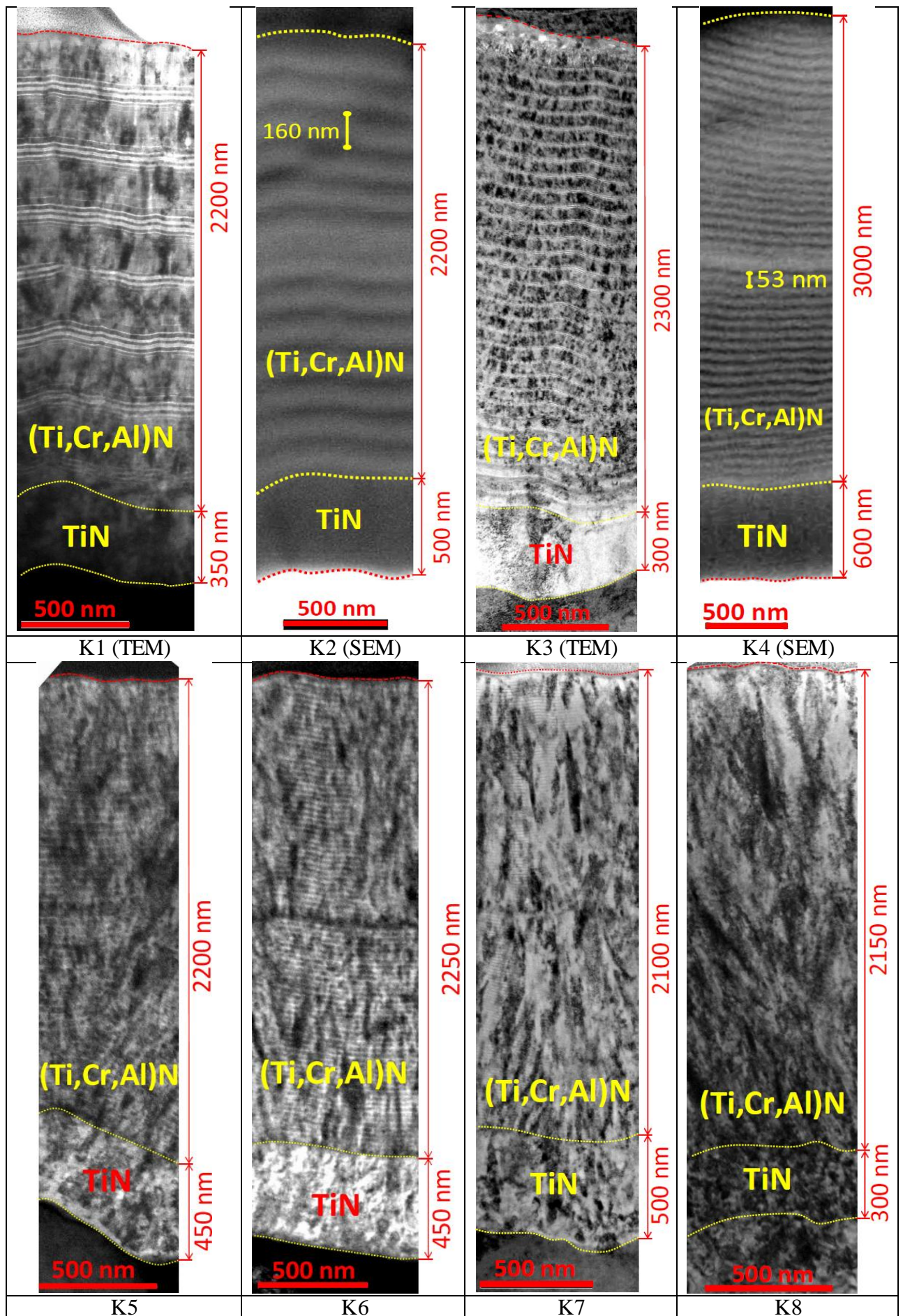
The nanostructure of the coatings under study (TEM).
