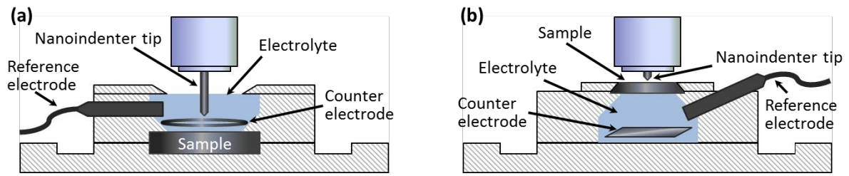
Figure 1 – Schematic of the built setups for in situ nanoindentation during electrochemical hydrogen charging: (a) front-side charging, and (b) back-side charging.
