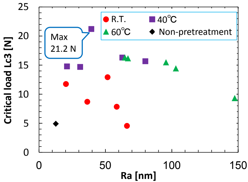
Figure 2 Relationship between arithmetic average roughness Ra and critical load (Lc3). PECVD TiC on aqua regia treated WC-Co.
