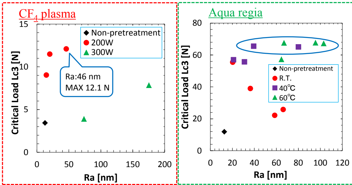
Figure 1 Relationship between arithmetic average roughness Ra and critical load (Lc3). Left: TiC on CF 4 plasma treated WC-Co, Right: TiC on aqua regia treated WC-Co.
