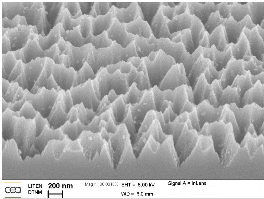
Figure 2 : SEM observation of moth-eye structure on glass substrate
