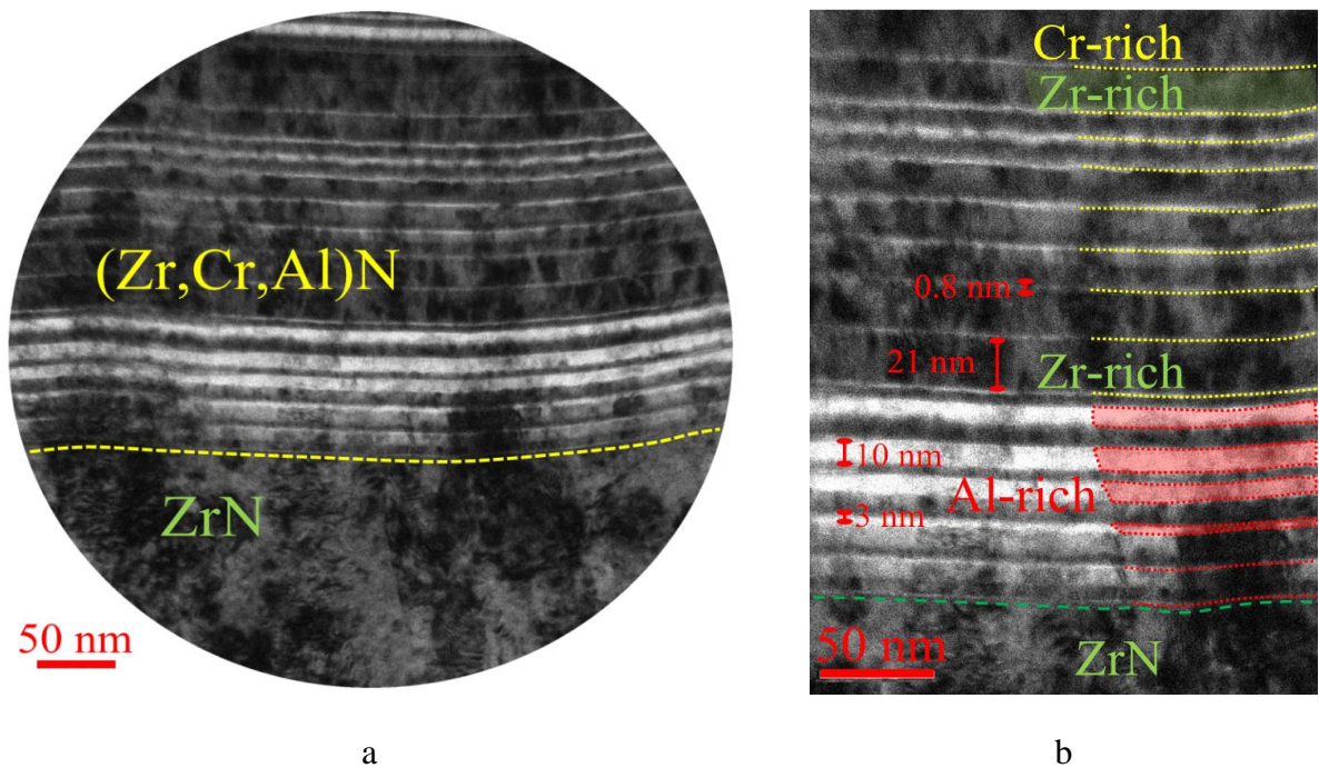
Fig. 2. Structure of nanolayers in the Zr-ZrN-(Zr,Cr,Al)N coating obtained using TEM.
