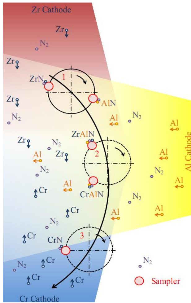
Fig. 1. Diagram to explain the deposition of the (Zr,Cr,Al)N layer on VIT-2 using the three-cathode system.
